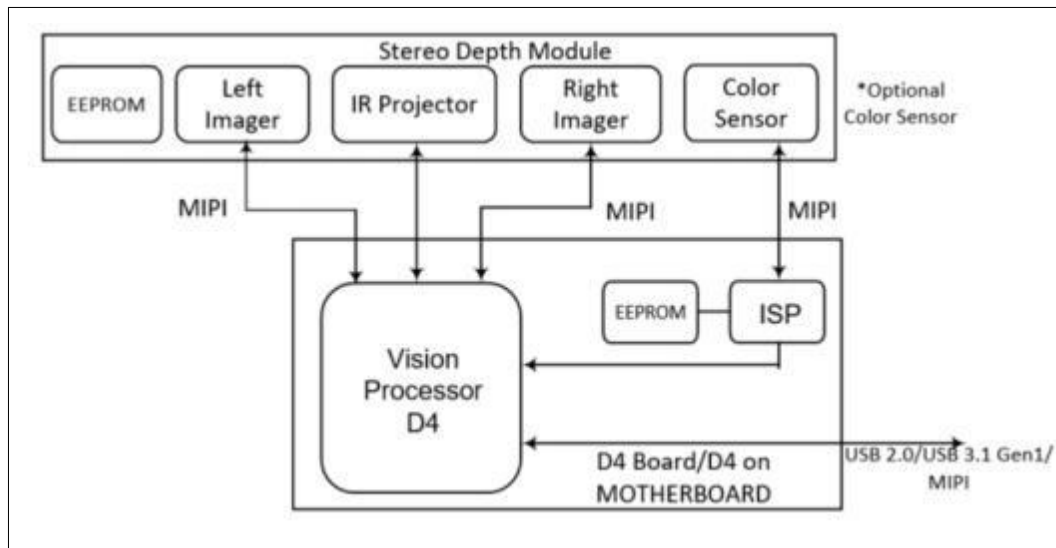
Figure 7-1. System Block Diagram - D415, D435, D435i, D455
