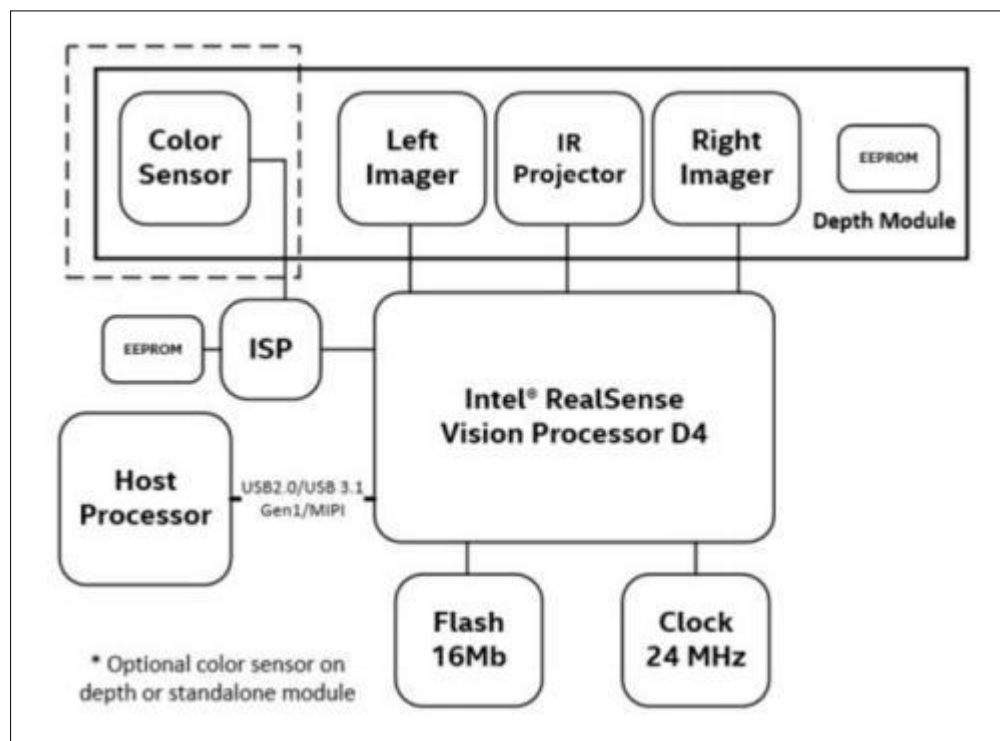
Figure 2-3. Vision Processor D4 Camera System Block Diagram
