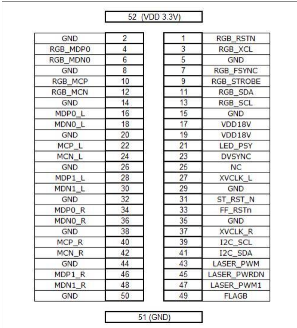
Figure 3-13. Depth Module Receptacle and Plug Connector Pin Position - D415, D435, D435i, D435f, D435if, D455, D455f, D456
