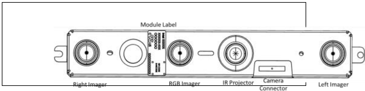
Figure 3-6. Stereo Depth Module (Intel® RealSense™ Depth Module D450)
