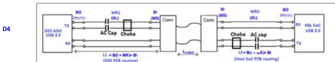
Figure 8-8. USB 3.1 Gen 1 Host to Vision Processor D4 Topology
