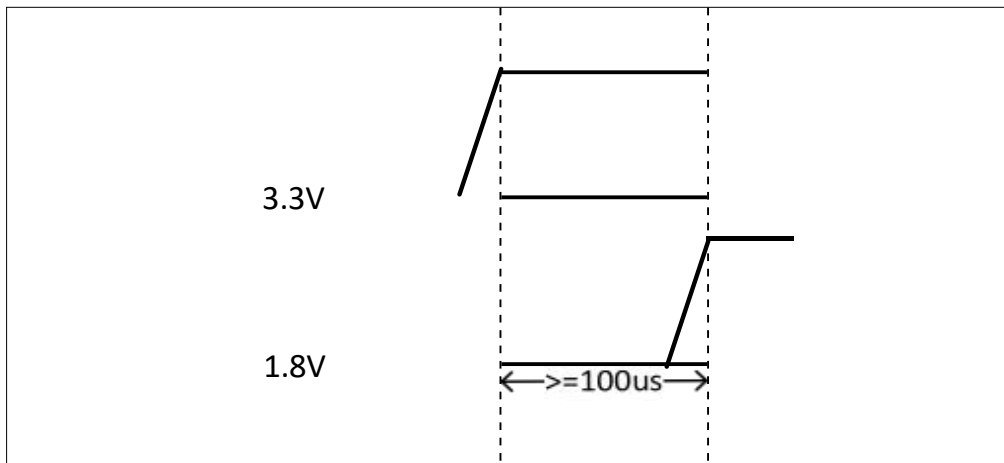
Figure 3-8. Stereo Depth Module Power Sequence
